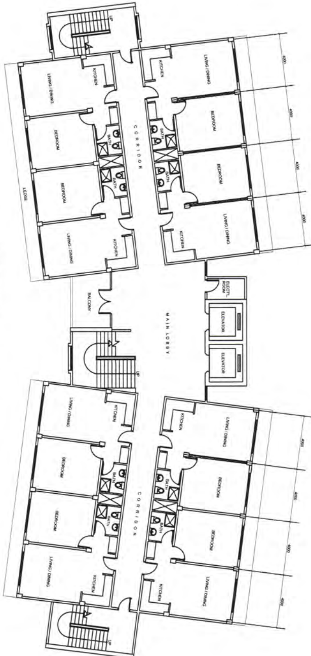
AREA = 710.48 sq m 1 TYPICAL 2ND-4TH FLOOR PLAN SCALE: 1:100 METERS A/02
