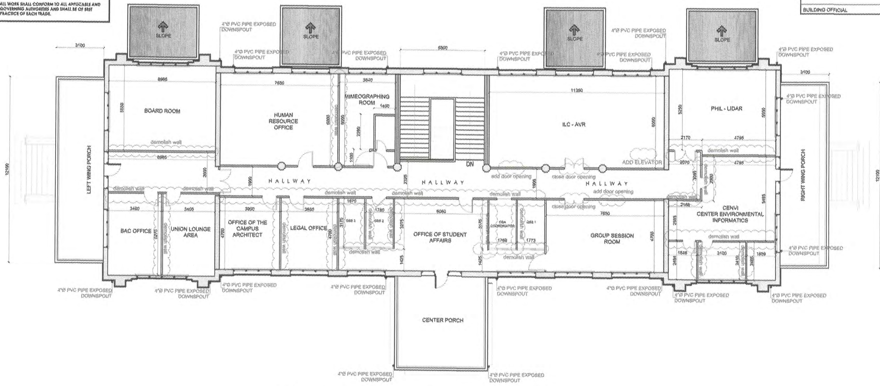
AS-BUILT + DEMOLITION PLAN ADMINISTRATION BUILDING SECOND FLOOR PLAN SCALE 1 : 150 METERS 1 A/03 0 0.5 1 2 4 10
