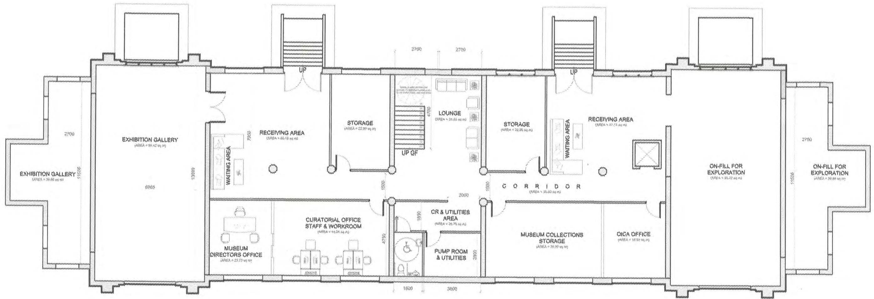
1 A/01 MUSEUM COLLECTIONS & EXHIBITION SPACES BASEMENT FLOOR PLAN SCALE 1 : 100 METERS
